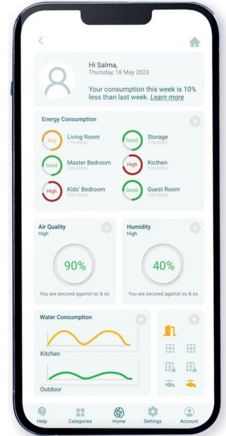
Home Analytics
