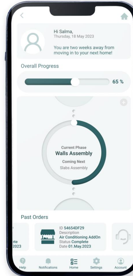
Tracking
