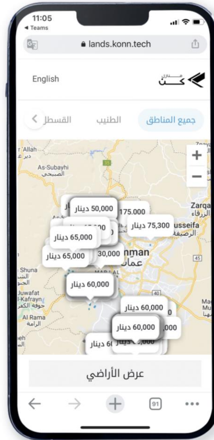
Land Selector
